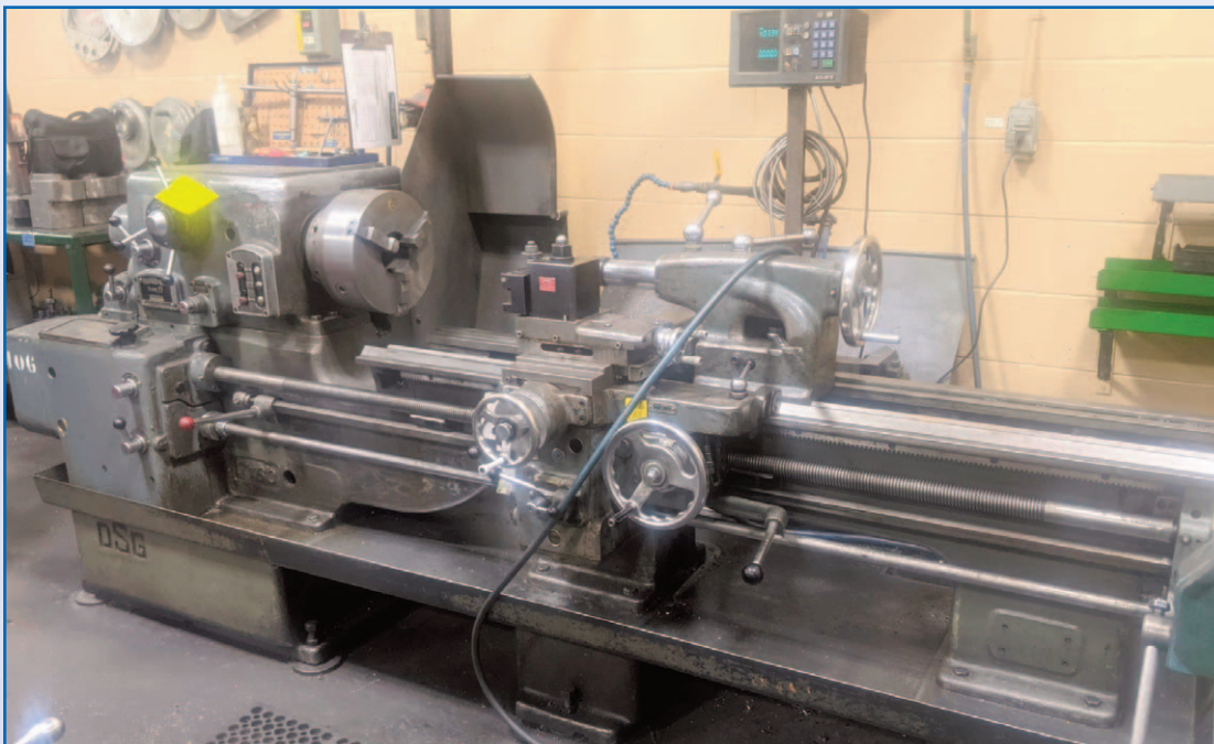
DEAN SMITH AND GRACE 17 ENGINE LATHE
